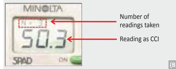
Figure 9.1. Using the Minolta SPAD-502 chlorophyll meter: (A) the main parts of the instrument; (B) measuring a flag leaf at the mid-point, ensuring that the midrib or main vein is not in line with the indent on the instrument, showing the chlorophyll concentration index (CCI) reading; and, (C) the 'average mode', and 'calibration mode'.
