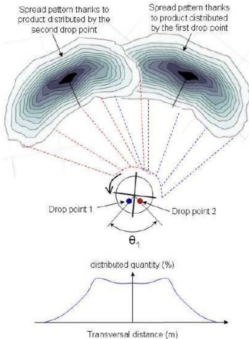
Fig 9: Consequences of different space interval between the two drop points on the spread pattern and on the transverse curve.
