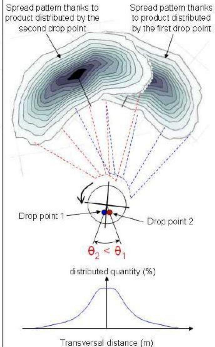
Fig 9: Consequences of different space interval between the two drop points on the spread pattern and on the transverse curve.
