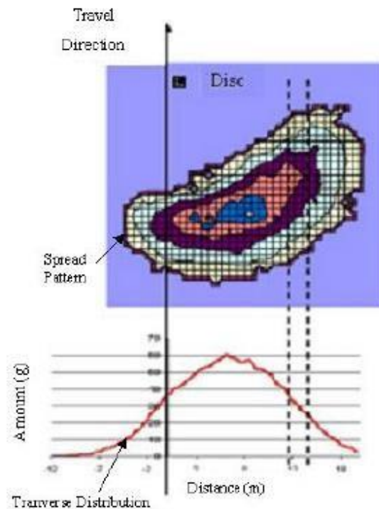
Fig. 1. Spread pattern (spatial distribution) and transverse distribution
