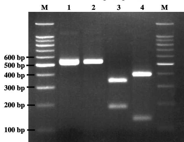
Fig. 12. PCR-restriction fragment length polymorphism (RFLP) pattern of the three Dothistroma species digested with the restriction enzyme AluI . A 100 bp marker (M) is on either side of the gel. Lane 1: uncut PCR amplicon (CMW 14822) used as a control; Lane 2: D. septosporum (CMW 6841) from Lineage I is not digested by AluI , Lane 3: the digested product of D. pini (CMW 14820) from Lineage II producing 2 bands of ~170 and ~350 in length; Lane 4: digested product of D. rhabdoclinis (CMW 12519) producing 2 bands of ~120 and ~400 bp in length.
